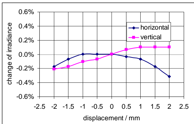
Figure 3. Change of the average irradiance while displacing a detector having 8 mm diameter aperture.
