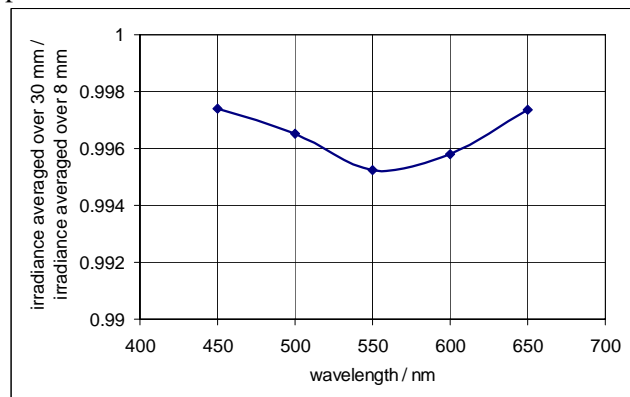
Figure 4. Ratio of irradiance averaged over two apertures diameter versus wavelength.
