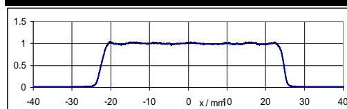
Figure 2. Irradiance field generated through imaging
