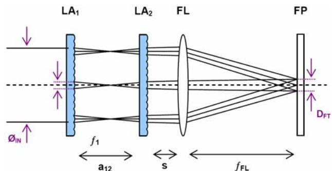
Figure 1. Imaging microlens array homogenizer
